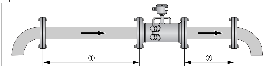
Figure 3-2: Recommended inlet and outlet for \geq \text{DN}100/4''
