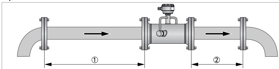
Figure 3-1: Recommended inlet and outlet for \leq \text{DN}80/3''
