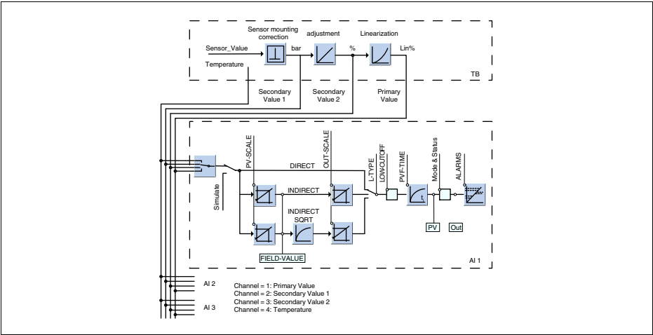
Рис. 28: Transducer Block VEGABAR 51 TB Transducer Block AI Function Block (AI =Analogue Input)
