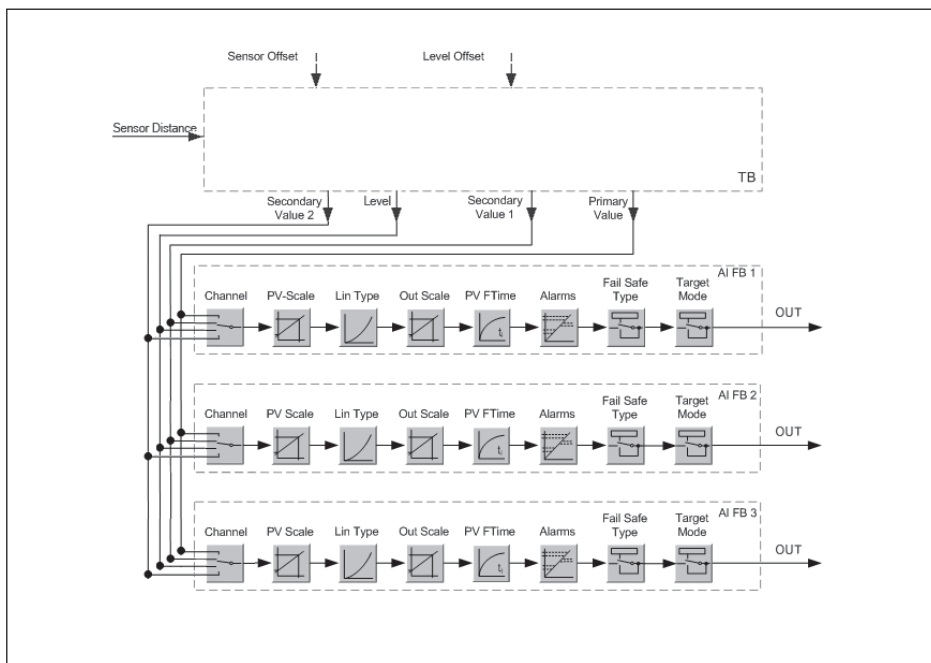
Рис. 57: VEGAPULS 62: Block diagram with AI FB 1 ... AI FB 3 OUT values
