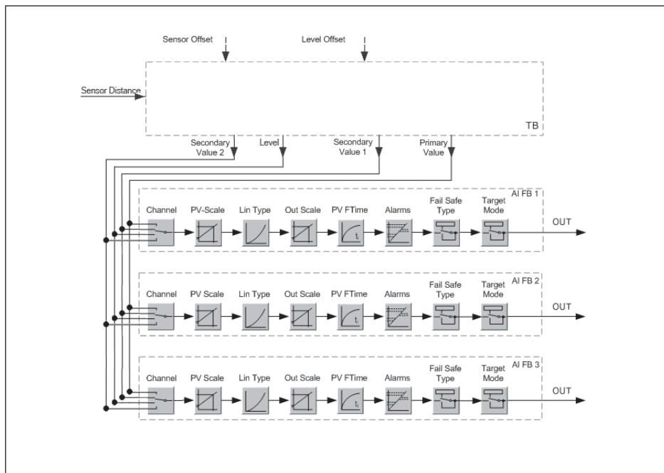
Рис. 48: VEGAPULS 63: Block diagram with AI FB 1 ... AI FB 3 OUT values
