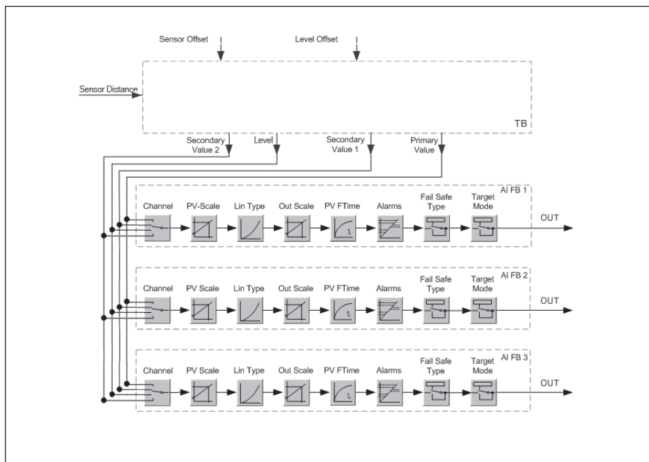
Рис. 46: VEGAPULS 65: Block diagram with AI FB 1 ... AI FB 3 OUT values
