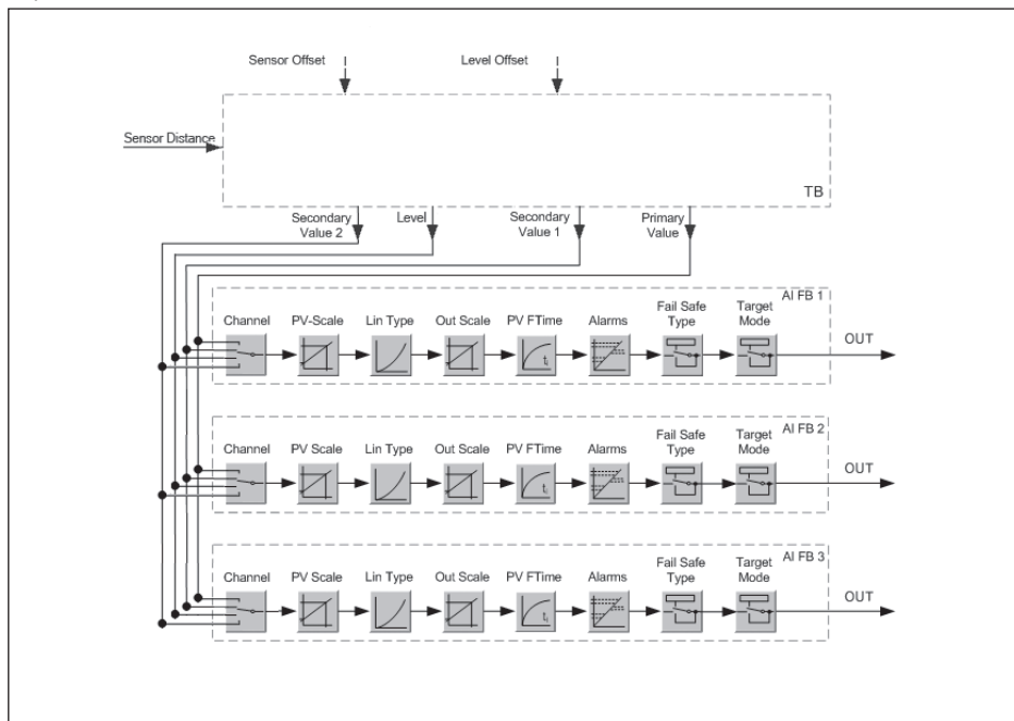
Рис. 29: VEGAPULS 66: Block diagram with AI FB 1 ... AI FB 3 OUT values
