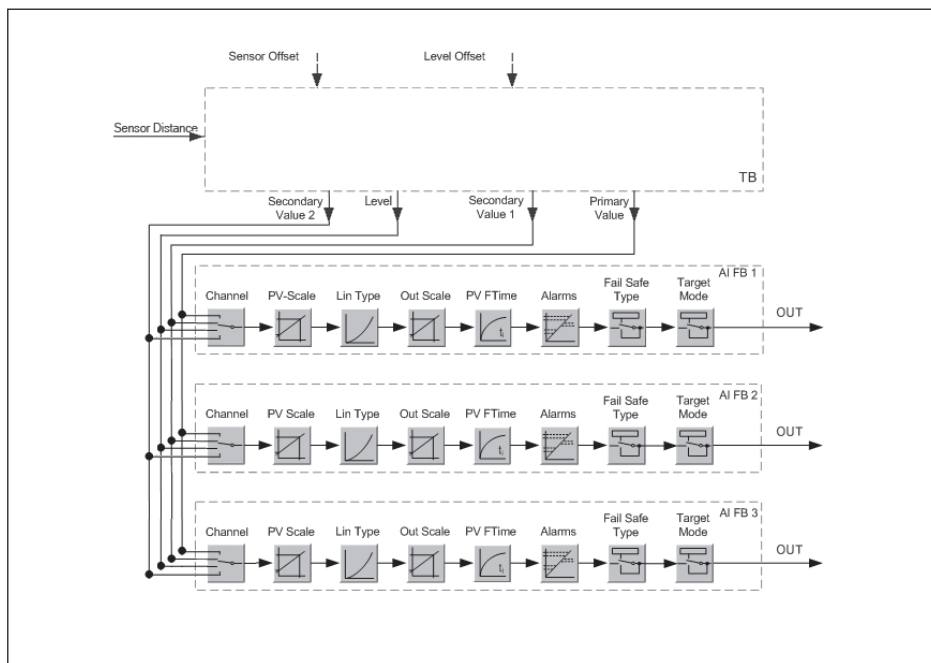
Рис. 50: VEGAPULS SR 68: Block diagram with AI FB 1 ... AI FB 3 OUT values
