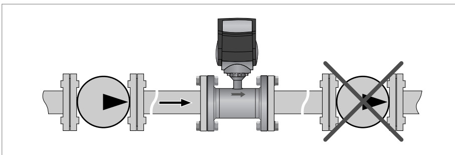
Figure 3-11: Recommended installation: after pump
