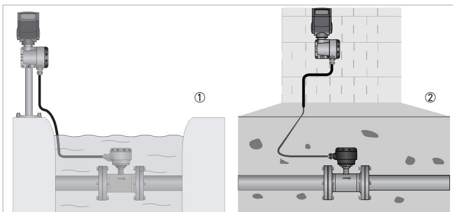
Figure 3-12: IP68 versions
