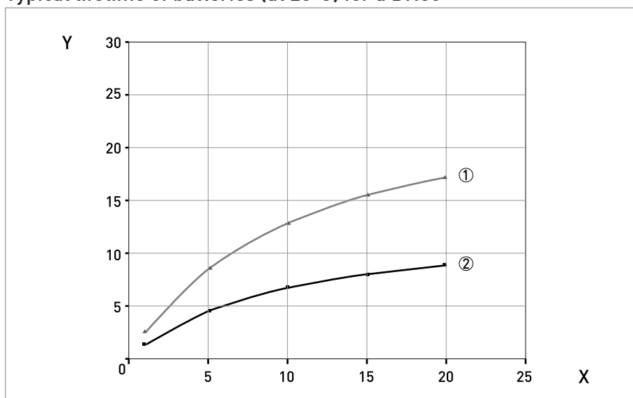
Figure 2-6: X = Measuring interval in seconds, Y = typical lifetime in years
