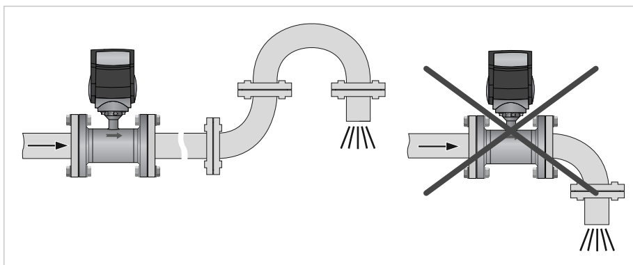
Figure 3-6: Installation in front of an open discharge
