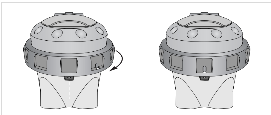
Figure 3-15: Closing of IP68 housing
